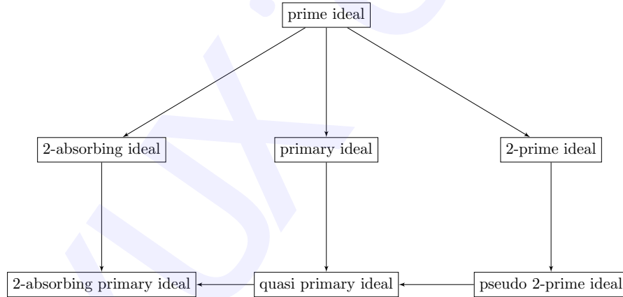
FIGURE 1. Pseudo 2-prime ideals vs other classical ideals
