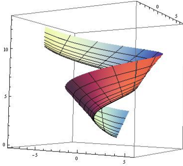
FIGURE 3. Canal surface \mathbb{M}_+^3 with r(s) = s .
